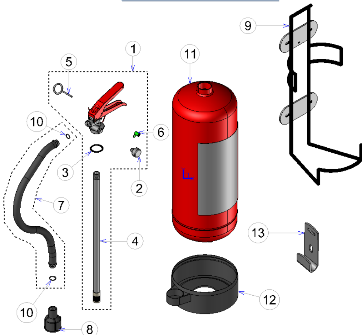
Couple de serrage de la vanne 30-55 DaN.m - Fastening couple of the valve 30-55 DaN.m
